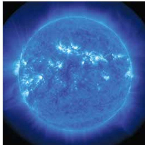
Extreme UV from the Solar Dynamics Observatory
