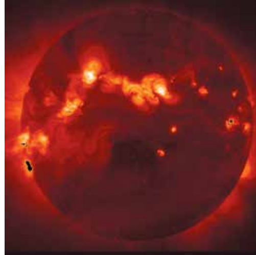
X-rays from Hinode spacecraft
