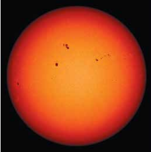
Visible light from the Solar Dynamics Observatory
