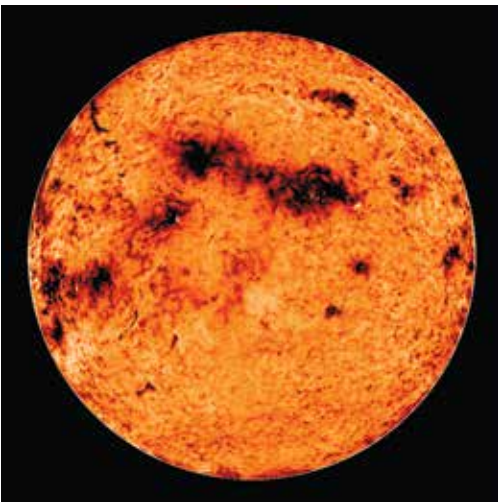
Infrared from National Solar Observatory
