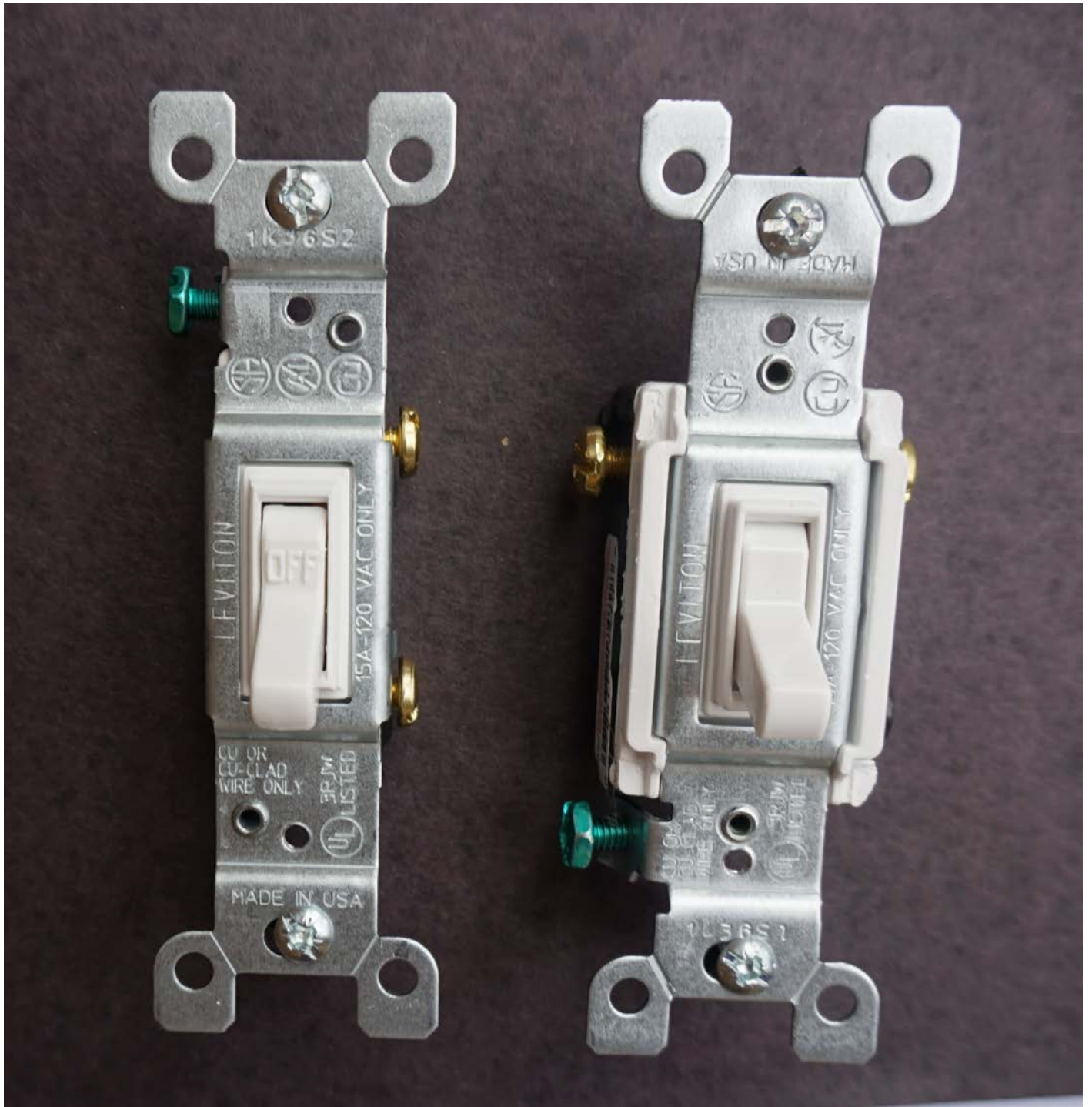
Figure 8.11. Single and Two-Way Switches
