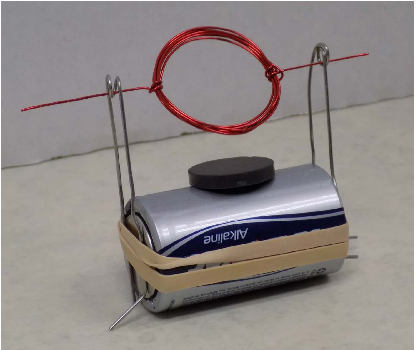
Figure 8.19. Homemade Electric Motor
