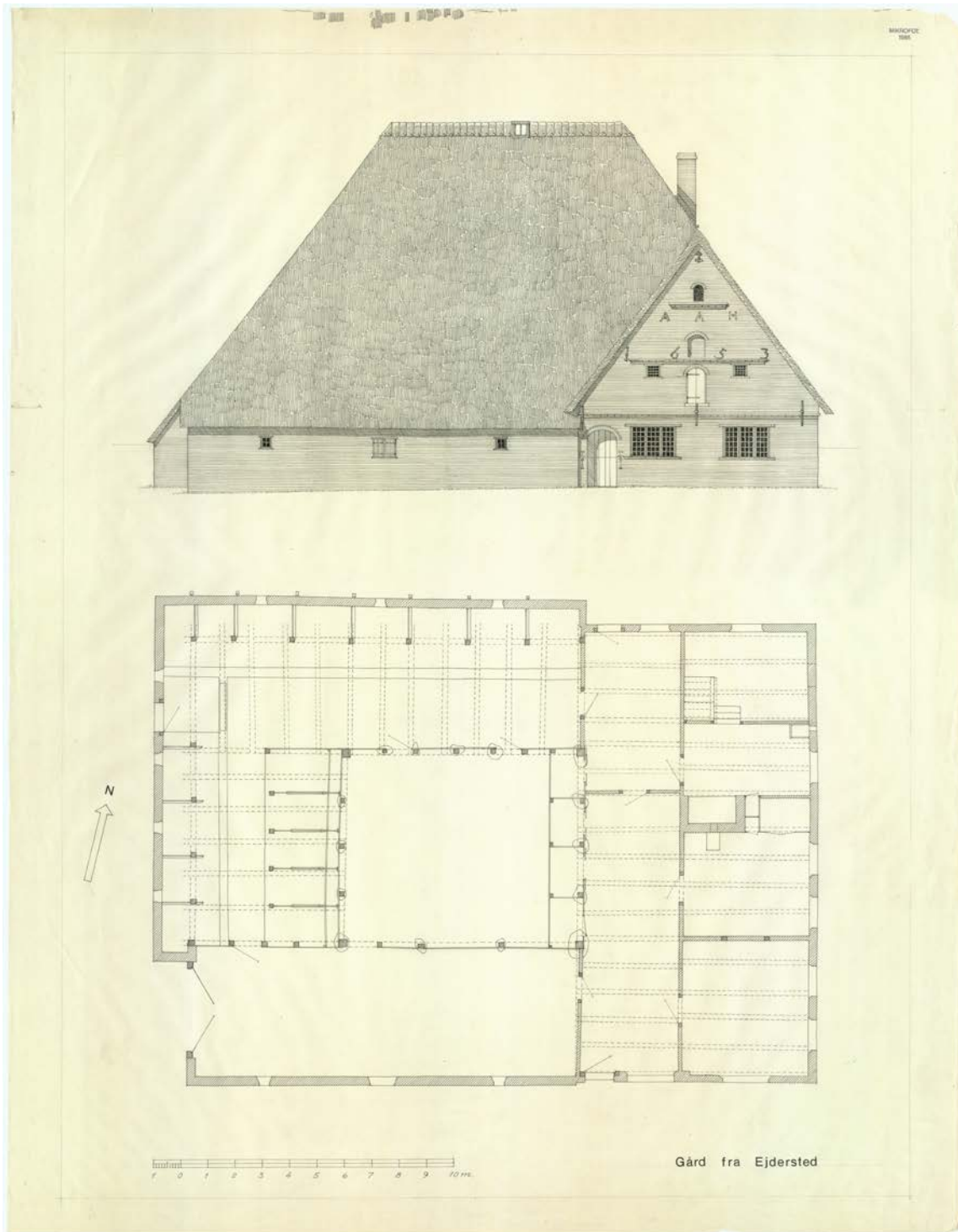
Figure 5.3. Building Blueprint
