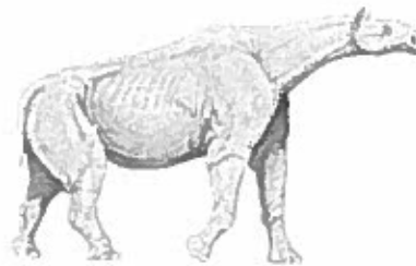
Miocene – 20 mya
