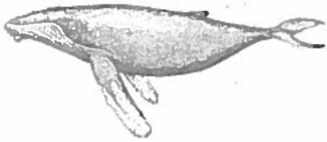
Quaternary – 1 mya
