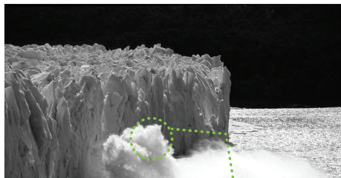
Calving Glacier
