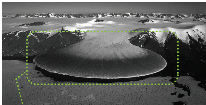
Piedmont Glacier
